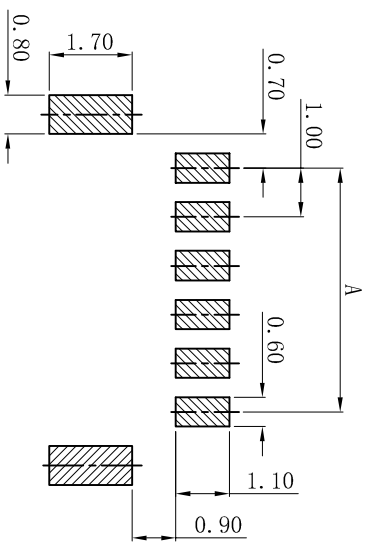
P.C.B LAYOUT: TOP VIEW TOLERANCE: ±0.05mm
