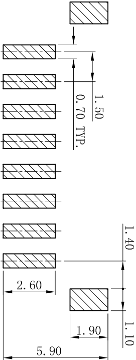
P.C.B. LAYOUT TOLERANCE: ±0.05mm
