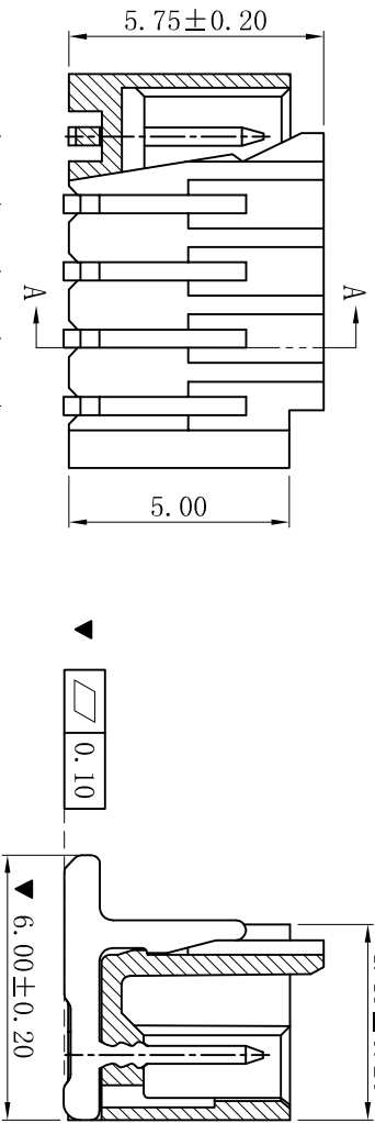
SECTION: A-A
