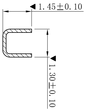
SECTION: C-C
