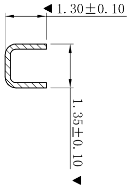
SECTION: D-D
