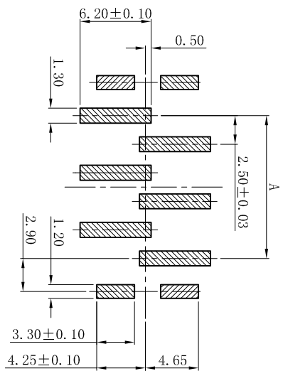
P.C.B LAYOUT: TOP VIEW TOLERANCE: ±0.05mm
