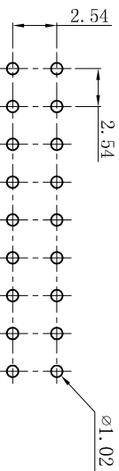
P. C. B LAYOUT
