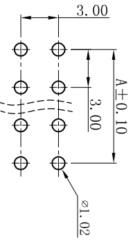
P.C.B. LAYOUT: TOP VIEW TOLERANCE: ±0.05mm
