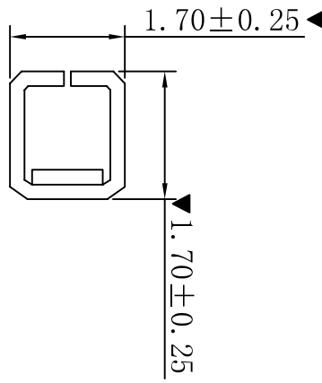
SEC:C-C
