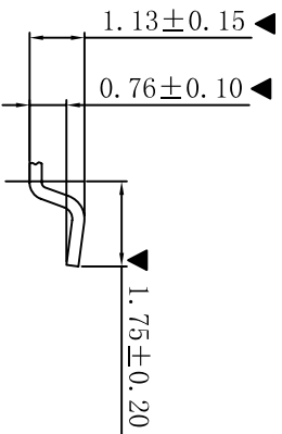
SEC:C-C
