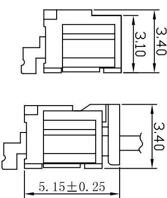
Mating Height Drawing
