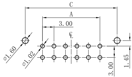
P. C. B LAYOUT: TOP VIEW TOLERANCE: ±0.05mm
