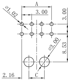
P.C.B LAYOUT: TOP VIEW TOLERANCE: ±0.05mm Poles: 08P~24P
